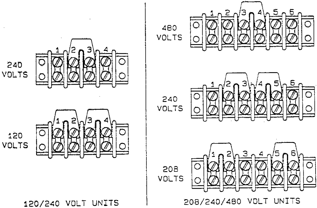
FIGURE 9.2.1A A.C. VOLTAGE SELECTOR BLOCKS
